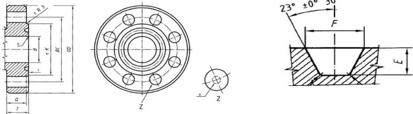
(Table-1B) _ Measurements For Chock Manifold Gate Valve Flange All Dimension In MM
