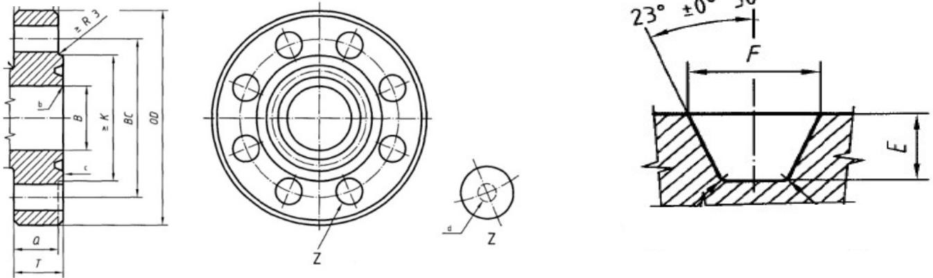
(Table-1A) _ Measurements For Chock Manifold Gate Valve Flange
