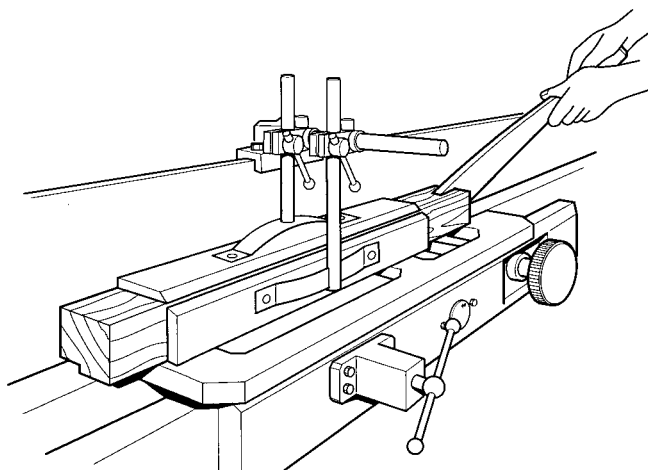
Figure 4 A push stick in use as a woodworking machine
